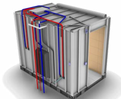
Distribution cabinet.
